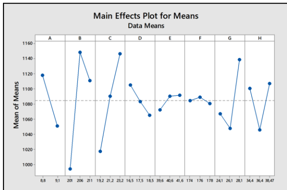
Fig 7: Main Effects for S/N Ratios Pipe Ring Flexibility
